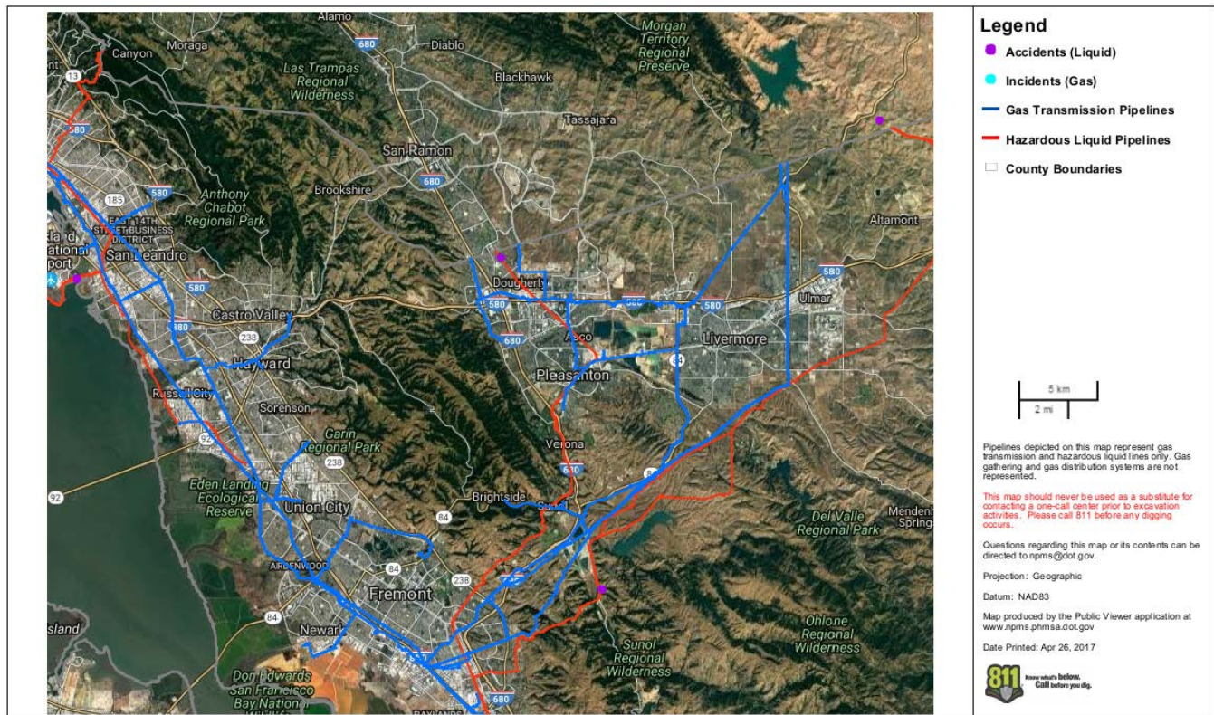
Figure 15-2. Gas Transmission and Hazardous Liquid Pipelines Near the Planning Area
