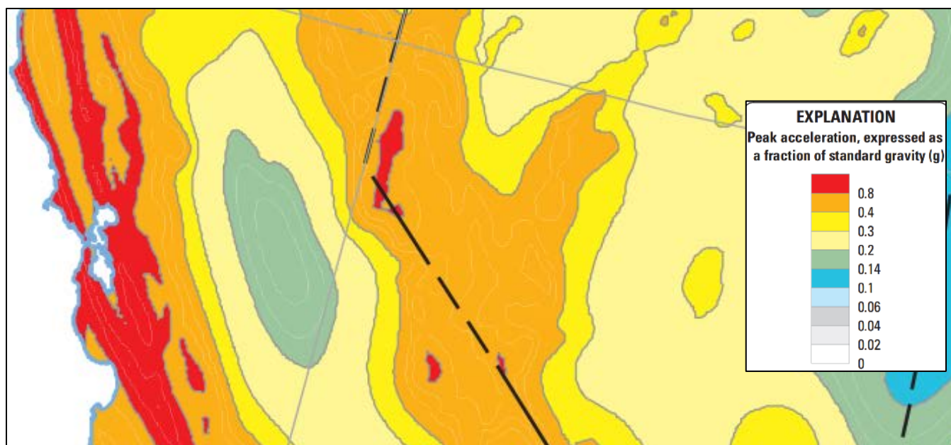
Figure 8-11. PGA with 2-Percent Probability of Exceedance in 50 Years
