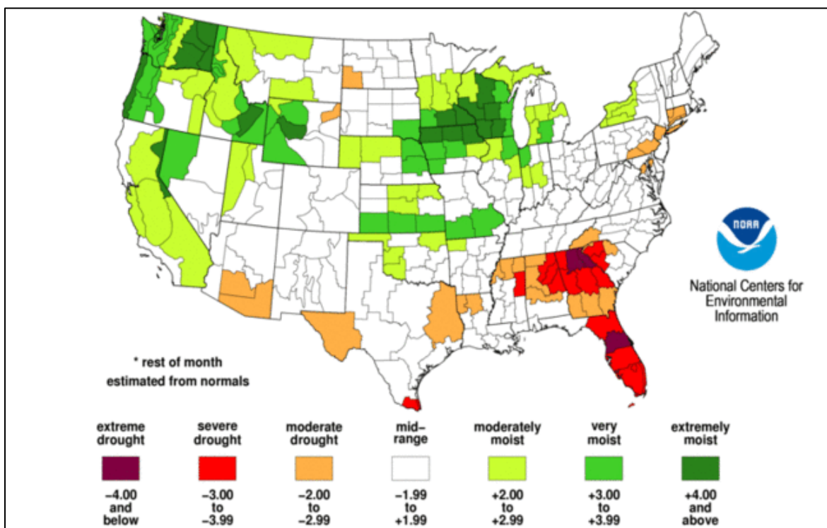
Figure 7-3. Palmer Drought Index through May 20, 2017
