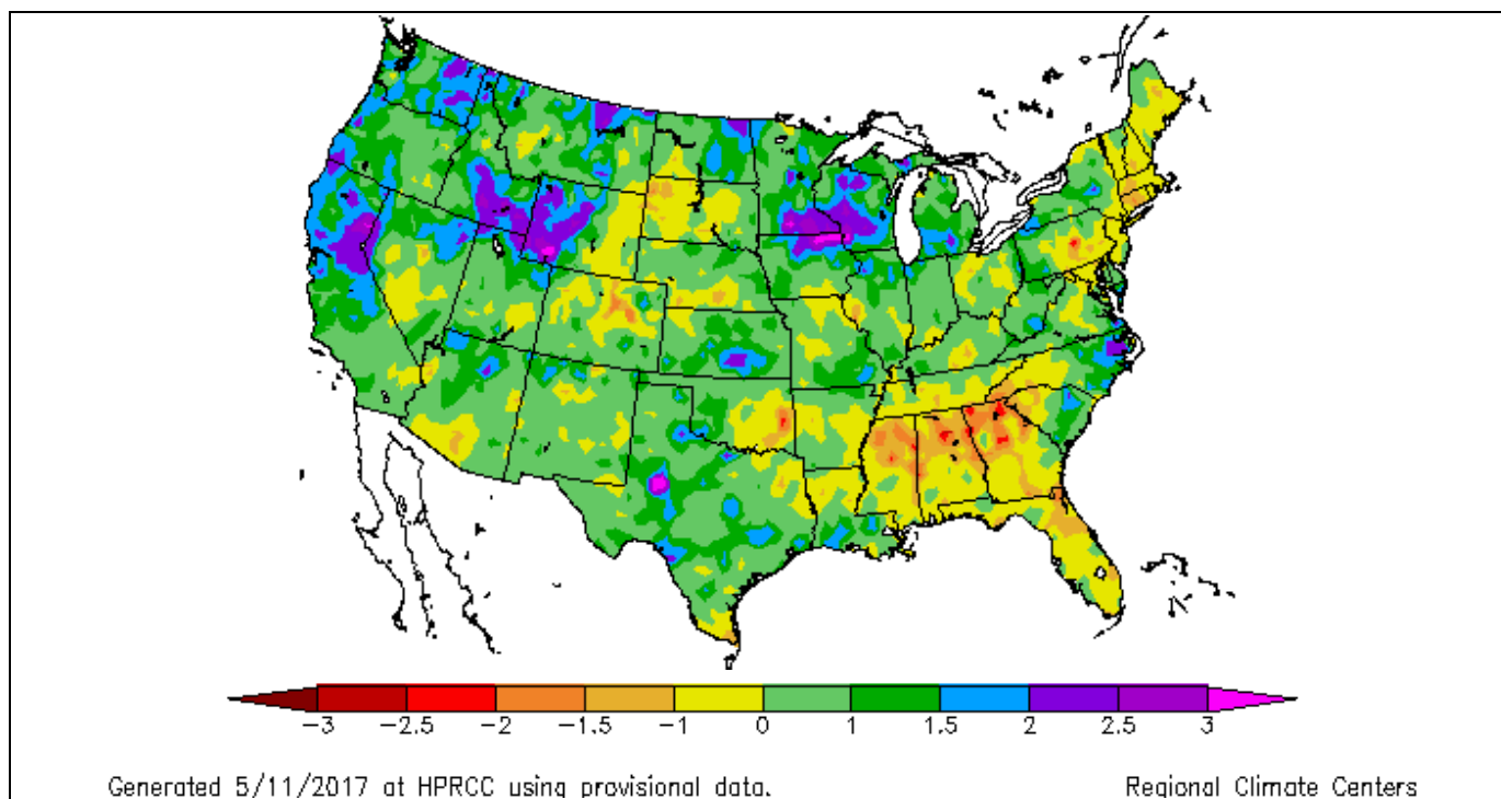
Figure 7-5. 12-Month Standardized Precipitation Index (May 1, 2016 – April 30, 2017)
