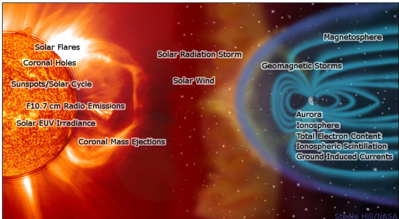
Figure 11-2. Space Weather Phenomena
