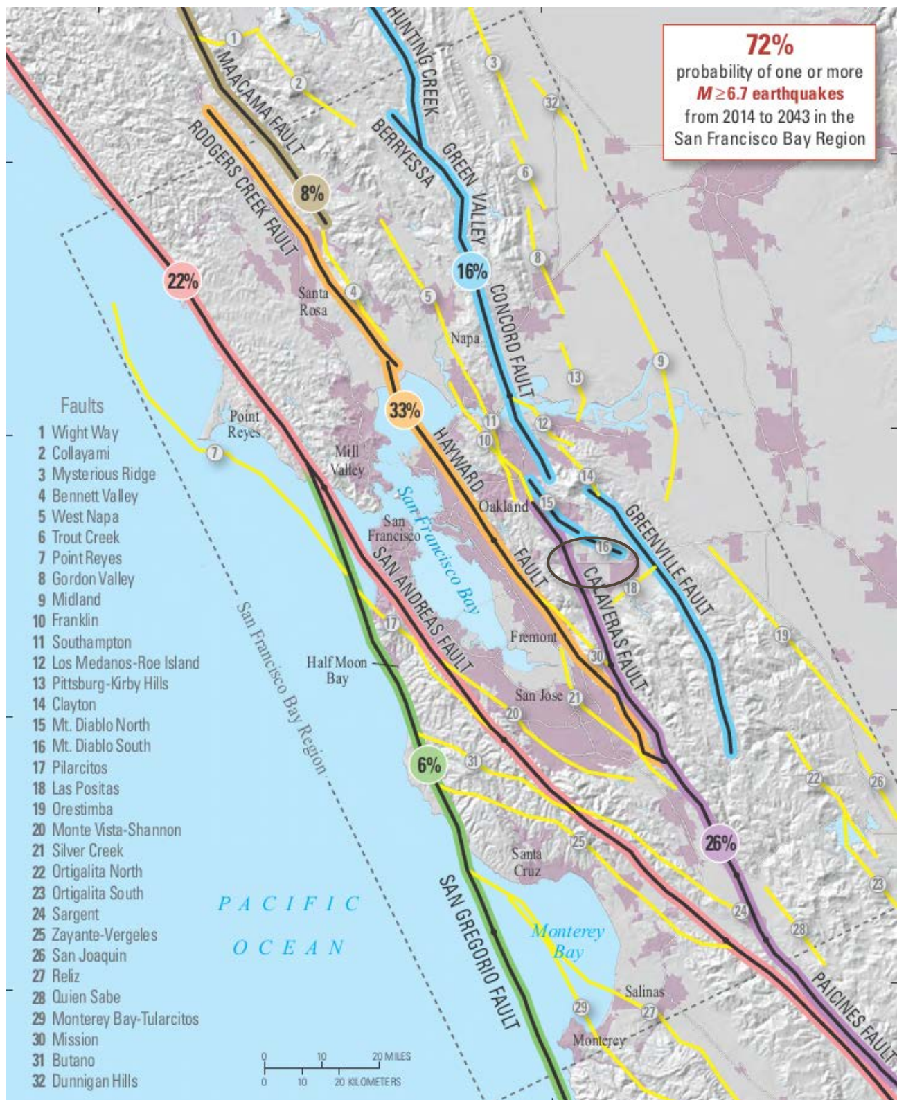
Figure 8-8. Significant Known Faults in the Bay Area
