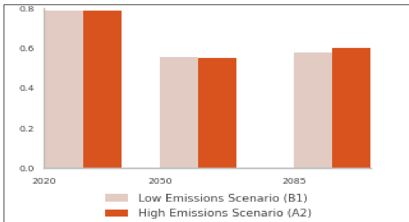
Figure 13-4. Projected Changes in Fire Risk, Relative to 2010 Levels
