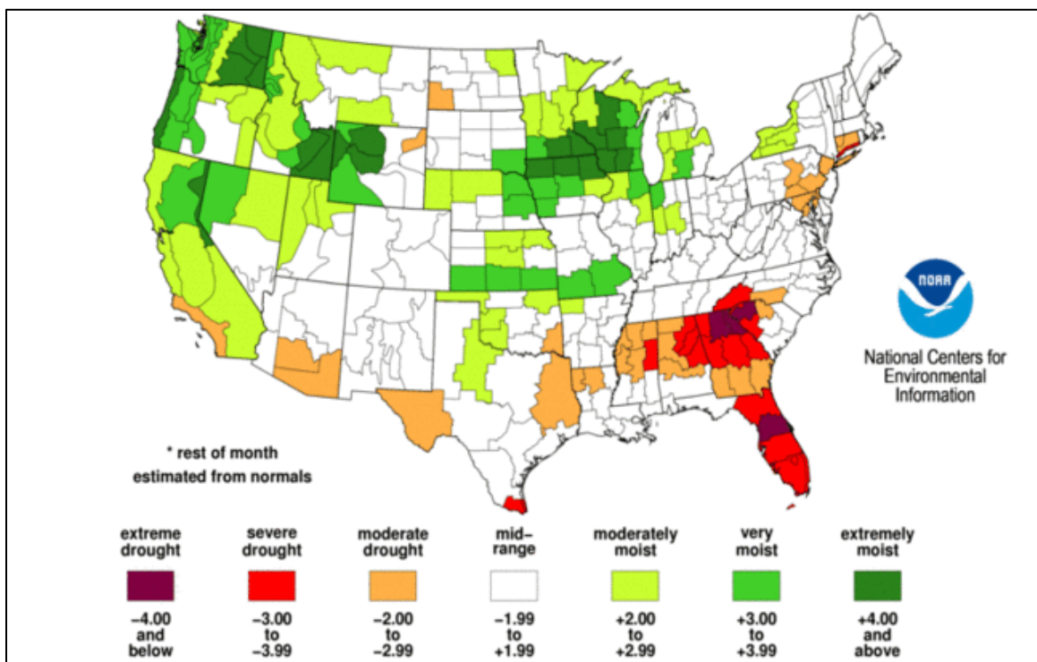
Figure 7-4. Palmer Hydrological Drought Index through May 20, 2017
