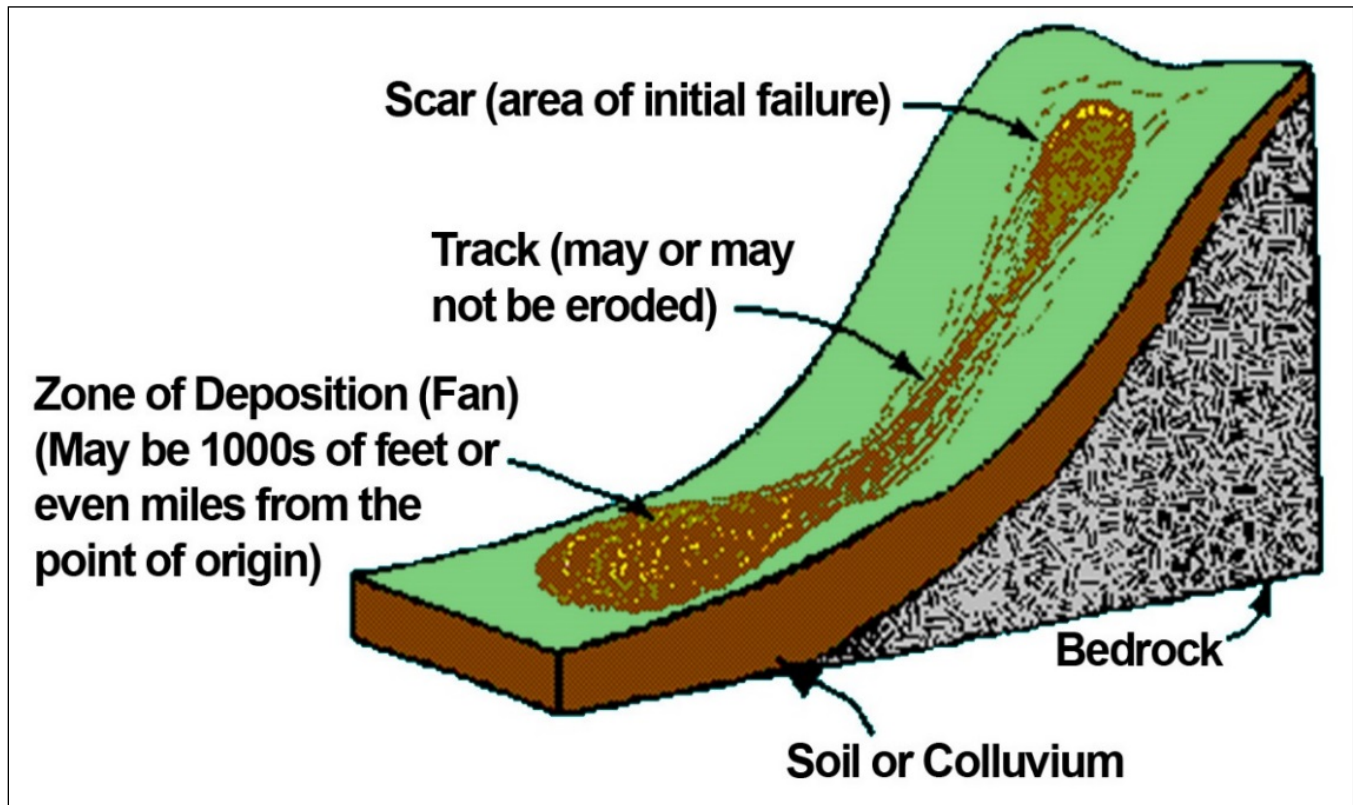
Figure 10-5. Typical Debris Avalanche Scar and Track
