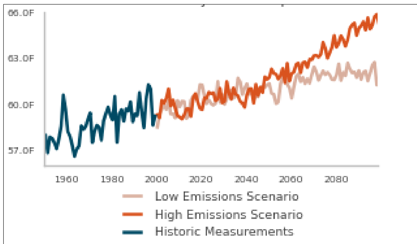
Figure 13-2. Observed and Projected Average Temperatures in Tri-Valley planning area
