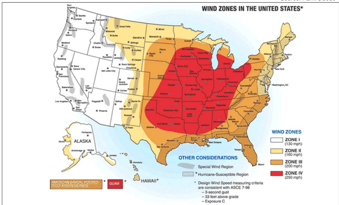
Figure 11-4. Wind Zones in the United States
