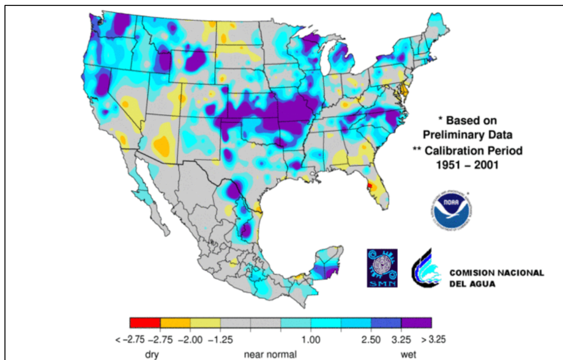
Figure 7-2. Palmer Z Index (April 2017)
